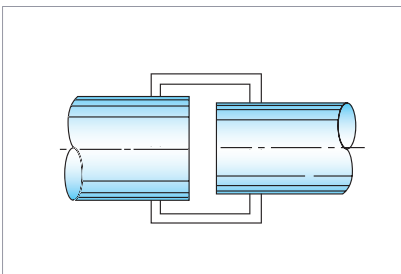
Absolutely no problems occur even if the pipe outer diameter (diameter) is either larger or smaller by about 2%.
