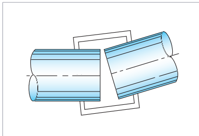
The center torsion is allowed up to 10° on both sides (one side up to 5°).
